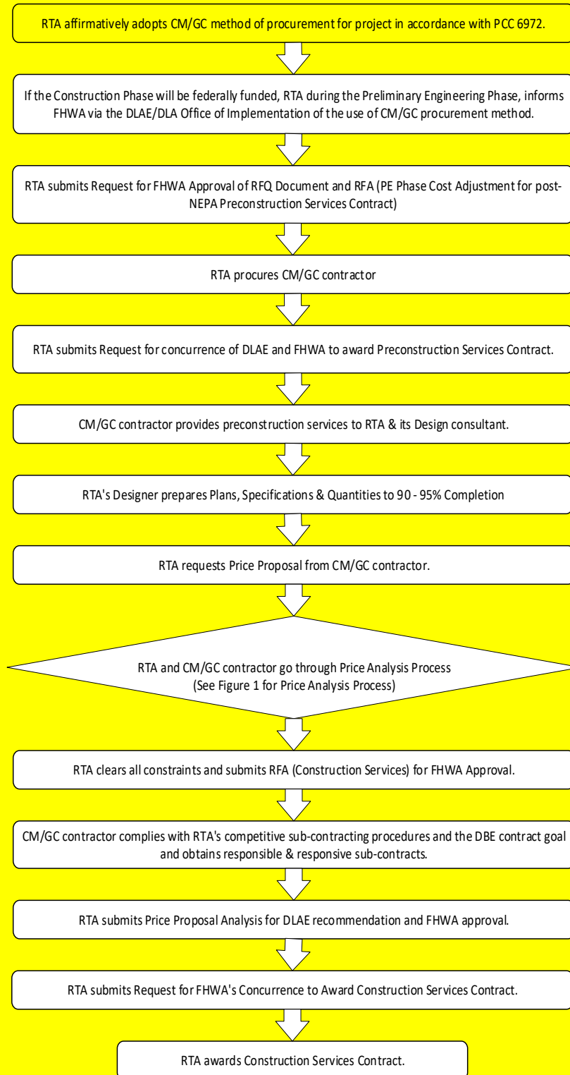
Figure 2 - CM/GC Process
